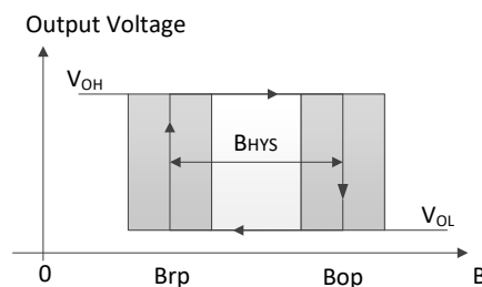
TO92S output status
